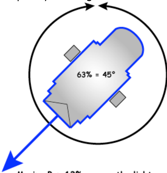
Moving Pan 13% causes the light to move to 45 degrees from Home.
